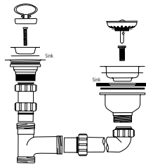
WASTE AND BOWL CONNECTION KIT CPK400
