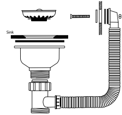
SQUARE OVERFLOW WASTE KIT CPK1900 - Chrome CPK2501 - Brushed steel
