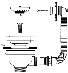
ROUND OVERFLOW WASTE KIT CPK501
