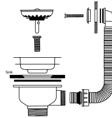
SQUARE OVERFLOW WASTE KIT CPK1501
