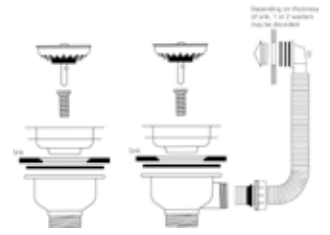
WASTE AND BOWL CONNECTION KIT CPK2701
