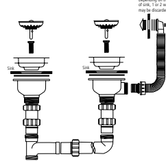
WASTE AND BOWL CONNECTION KIT CPK801
