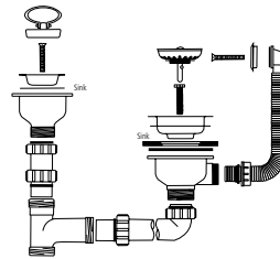
WASTE AND BOWL CONNECTION KIT CPK1101
